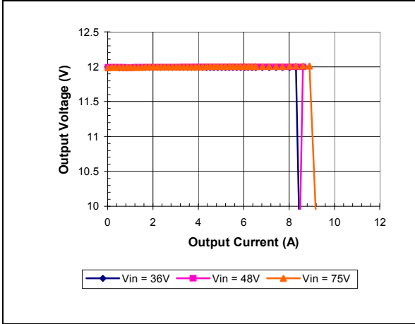
iEA48007A120V-000 Typical Output Current Limit Characteristics vs. Input Voltage at Ta=25 degrees.
